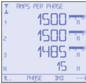
3-phase and neutral current display
